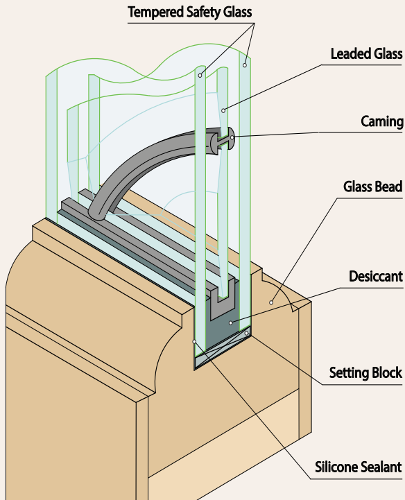
Cross Section of Insulated Leaded Glass
